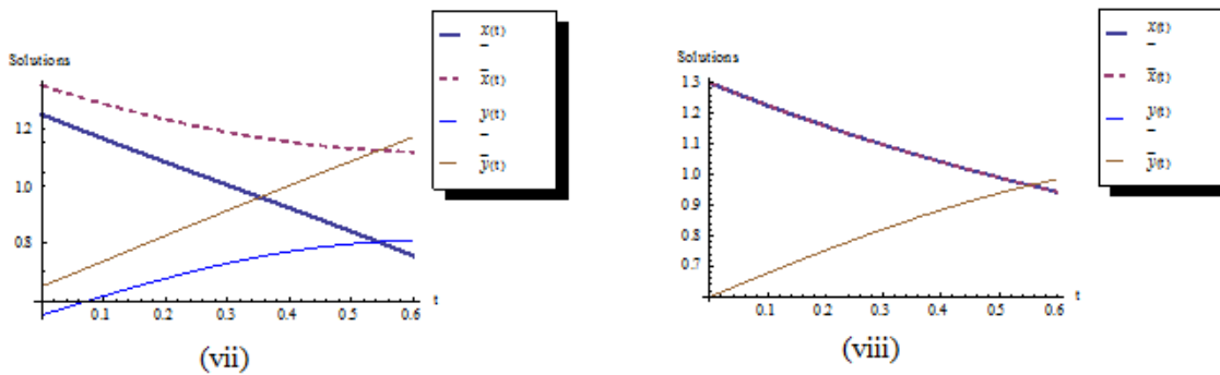
Figure 9. Interval solution of fractional predator-prey equations of Case 1 for \tilde{x}(t) and \tilde{y}(t) with \alpha = \beta = 1 at (vii) \gamma = 0.5 and (viii) \gamma = 1
