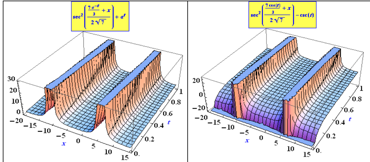
Figure 2. Plots of solutions to the BBM obtained in Case III and IV respectively
