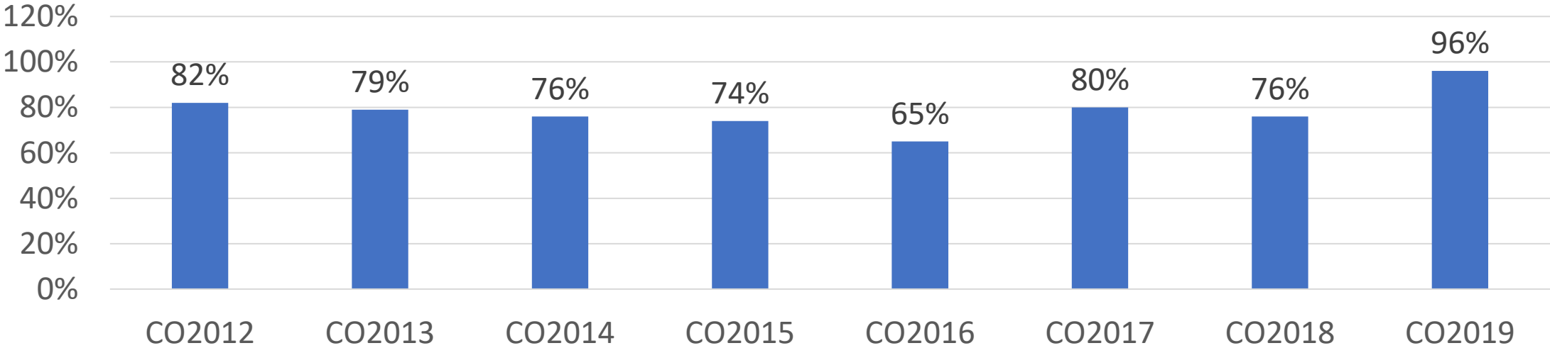
ELEG 1st Year Retention
