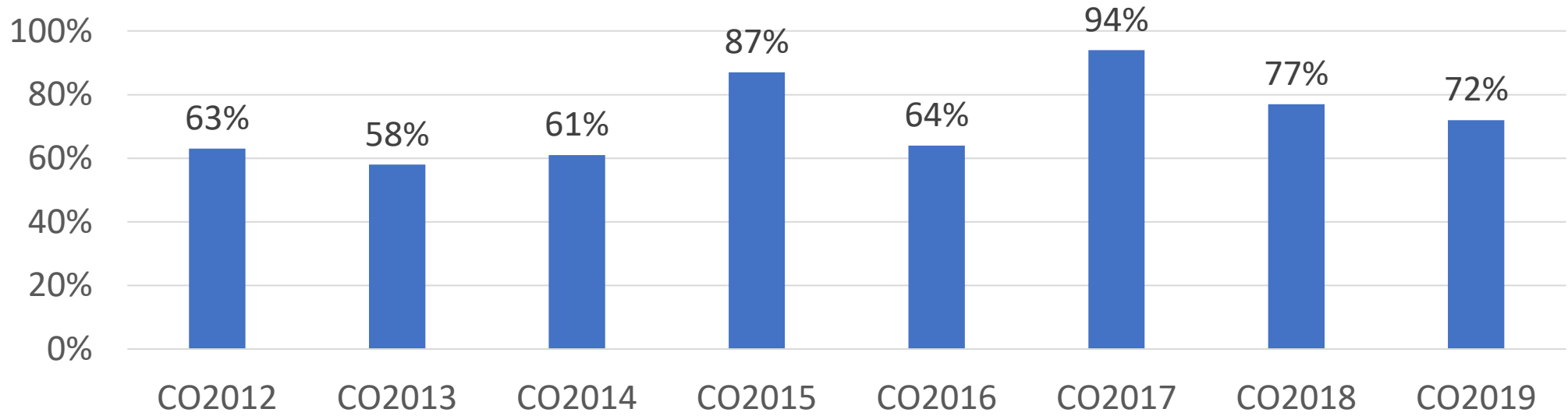
CPEG 1st Year Retention
