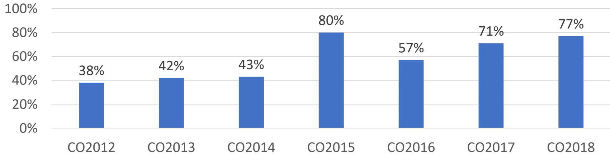
CPEG 2nd Year Retention
