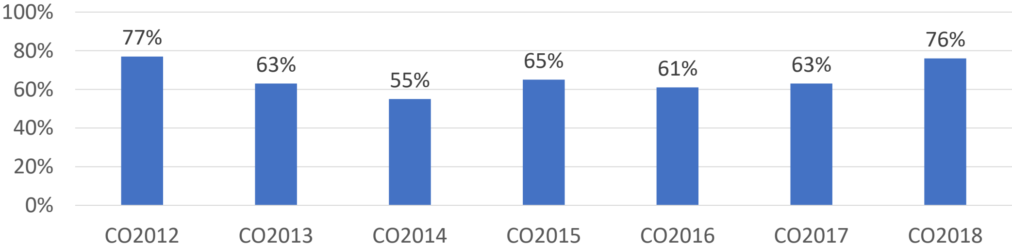
ELEG 2nd Year Retention
