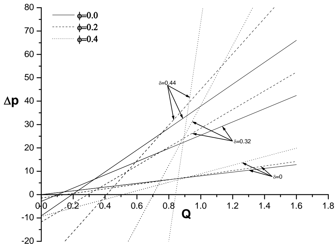
Fig.2 Variation of \Delta p with Q for different \phi and \delta .
