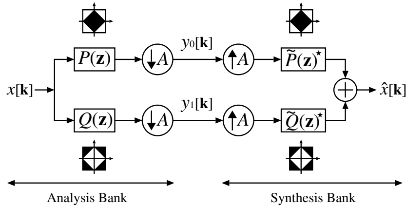
Fig. 1. An illustration for a PR QMF induced from a system of 2D quincunx scaling function \phi and wavelet \psi and their biorthogonal scaling function \tilde{\phi} and wavelet \tilde{\psi} .
